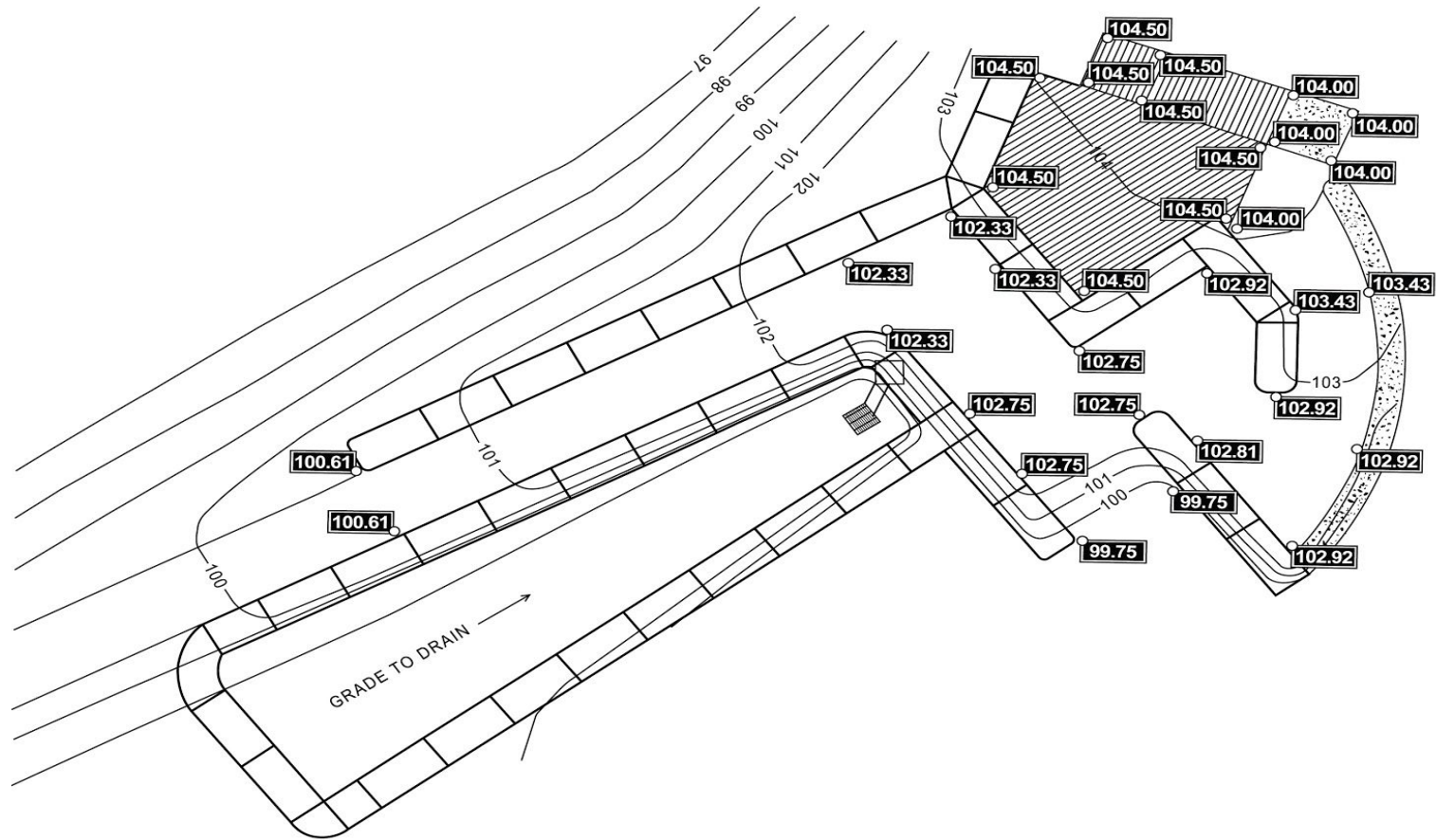
Figure 2.1 - Topographical Grade Map pinpointing slope and measurement data for the rear entrance of Fire Station Park.
